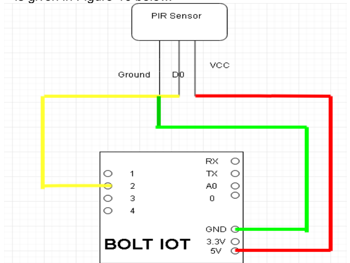
Fig -10: Circuit Design for Motion Detection
