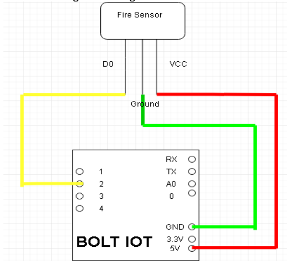
Fig -14: Circuit Design For Fire Detection
