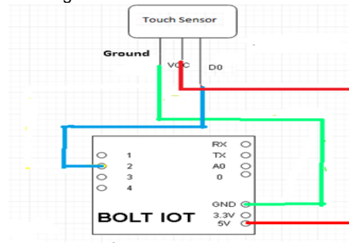
Fig -18 Circuit Design for Security Detection
