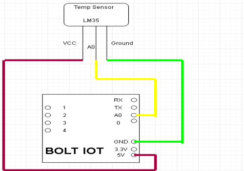
Fig -5: Circuit Design for Temperature Monitoring
