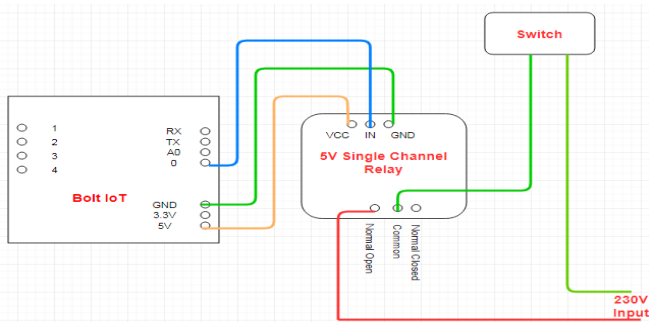
Fig -26: Circuit design for control Switch ON/OFF
