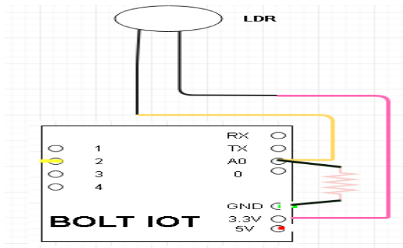
Fig -22: Uplink device circuit
