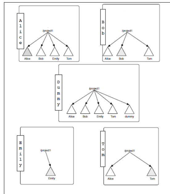
Fig Distributed approach.
