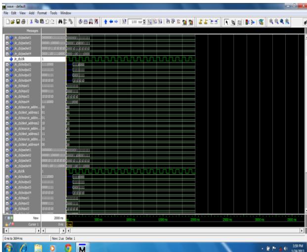
Fig.8 Reconfigurable 4x4 Crossbar switch ModelSim software tool waveform simulation.
