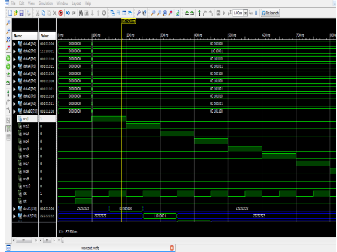
Fig.6 RTL simulation view of Reconfigurable Crossbar Switch
