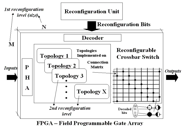
Fig.1 FPGA –Reconfigurable Crossbar Switch.
