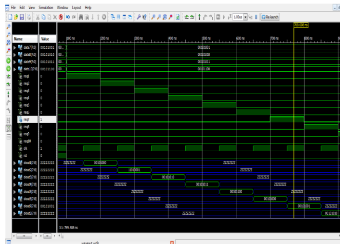
Fig.7 Reconfigurable 10x10 Crossbar switch Xilinx ISE 13.1 software tool waveform simulation.
