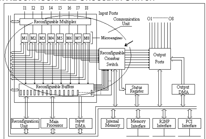
Fig.5 R2NP (Reconfigurable RISC Network Processor) architecture
