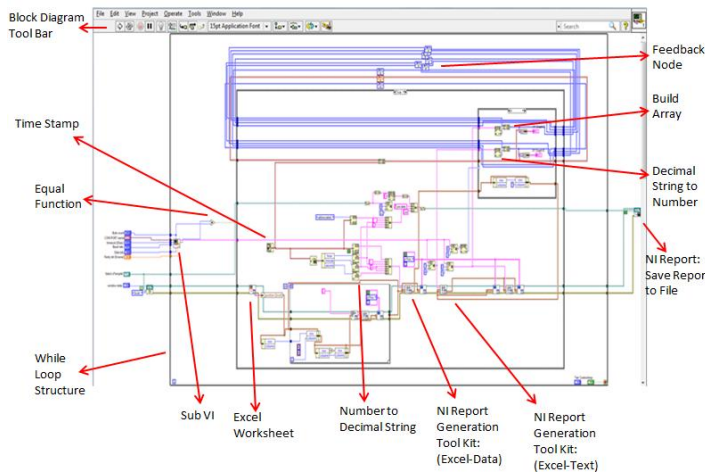
Fig 5. Block Diagram of the Complete System
