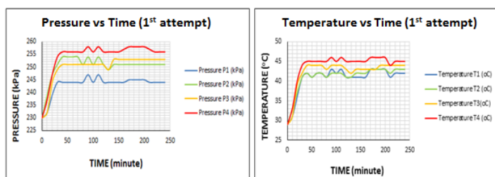
Fig 9. Pressure and Temperature Variation over Time during First 300km Attempt
