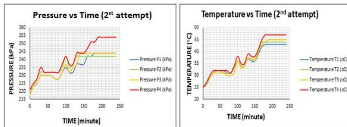
Fig 10. Pressure and Temperature Variation over Time during Second 300km Attempt
