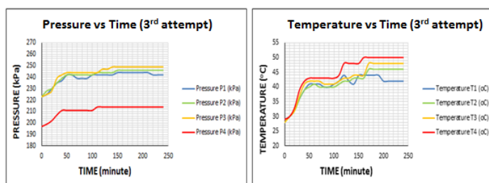
Fig 10. Pressure and Temperature Variation over Time during Third 300km Attempt
